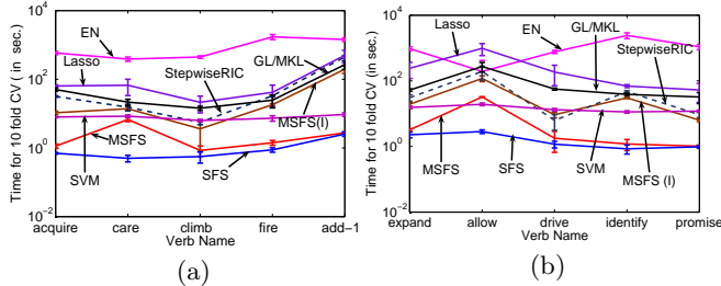
Figure 1: Graphs showing total running times for 10 fold CV (in seconds) for various methods for WSD Datasets. Note: The y-axes are drawn on log scale
